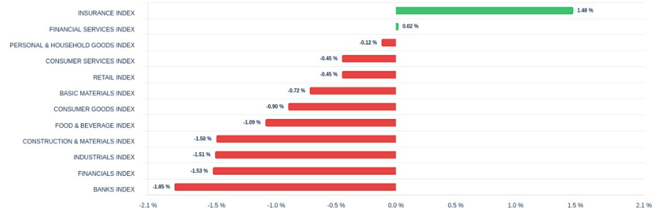
Daily Change of Sector Indices
